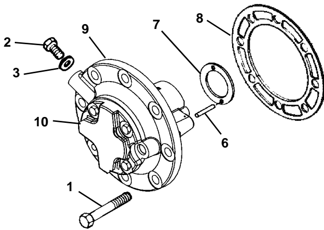
LOW PROFILE PUMP (NLO)
